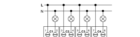
e Connection loads K.ENN.01O.20N.WO (4-fold)
