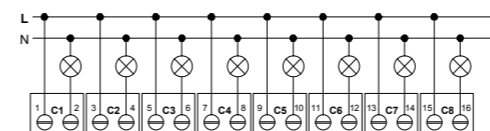
f Connection loads K.PAL.01O.20N.WO (8-fold)
